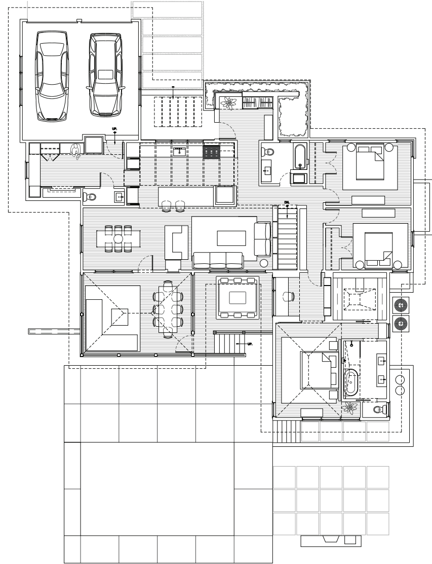
NEW GROUND FLOOR PLAN
